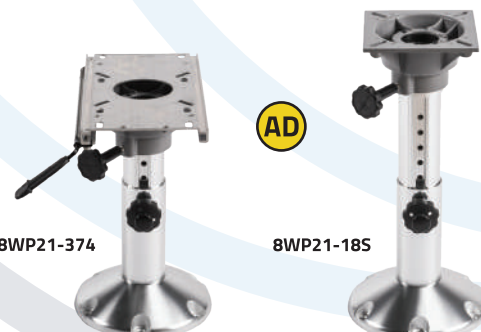
8WP21-374 ADJUSTABLE PEDESTAL W/ FORE & AFT SLIDE Features Adjusts from 12" to 18" Smooth, Thick Walled, Polished Anodized Aluminum 2 7/8" Diameter Pipe Locking Seat Mount w/ 360° Rotation 9" Diameter Base
