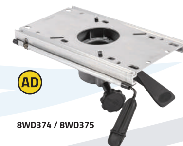
8WD374 FORE & AFT SEAT SLIDE Features Allows 5" of Fore & Aft Travel Fits 2 7/8" O.D. Pedestal Cast Aluminum Construction Injection Molded Plastic Handles 8WD375 Fits 2 3/8" O.D. Pedestal
